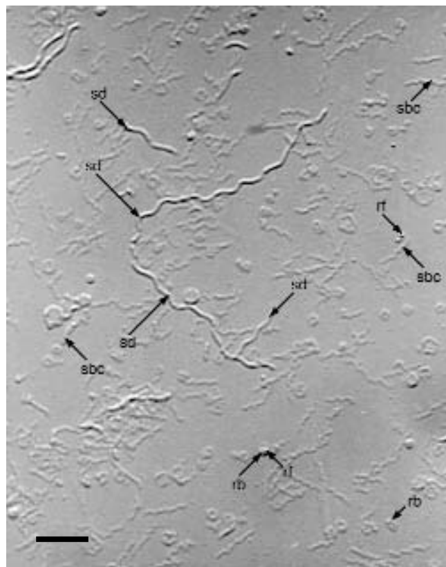
Fig. 1 Spirosymplokos deltaeiberi (sd) from Spain, showing detectability of these large spirochetes when live. Nomarski DIC in mixed enrichment culture with Spirochaeta bajacaliforniensis (sbc). Round bodies (rb), refractile structures (rf), bar = 10 µm
