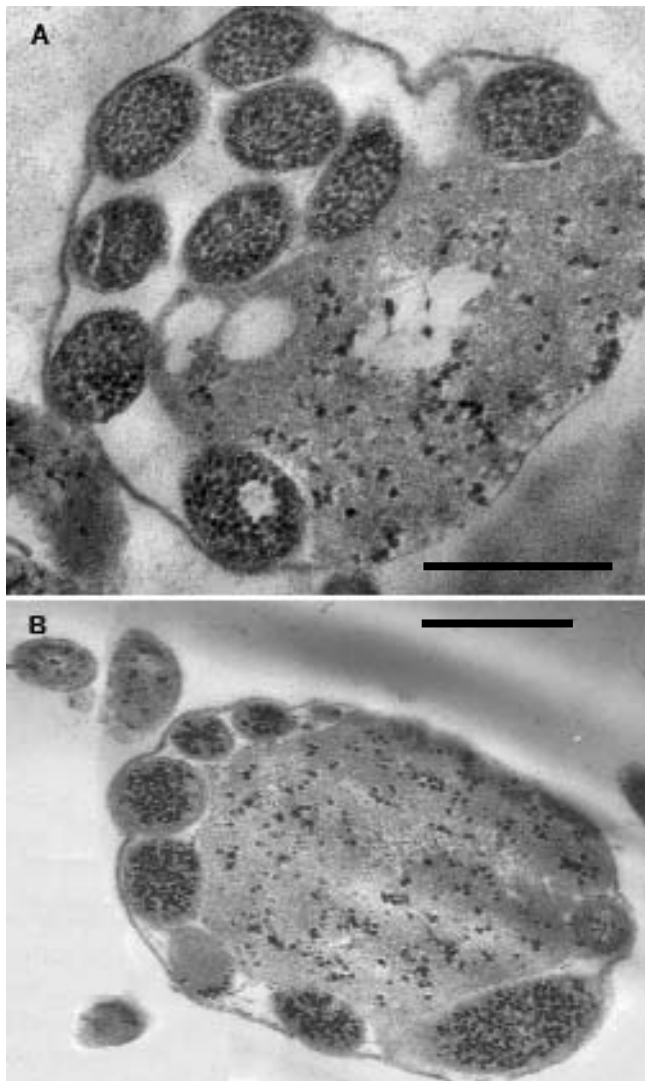
Fig. 4 Large composite spirochetes from Sippewissett salt marsh (bars = 5 \mu\text{m} ). (A) Parental protoplasmic cylinder disintegrating in healthy rounded composite granulated spirochete round body. Single spirochete emerging at lower left. (B) Variable diameter (lower right) of composite spirochete in rounded membrane-bounded body
